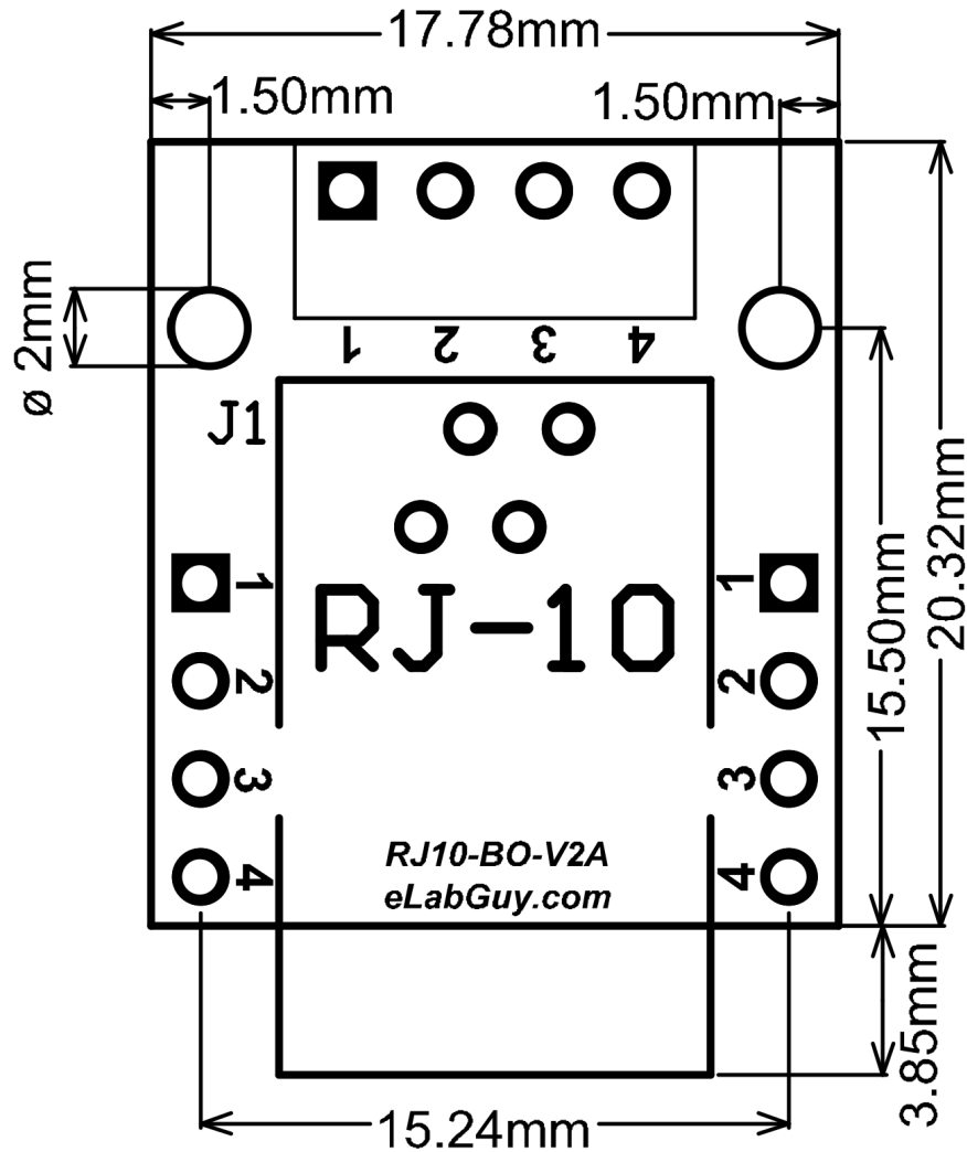
RJ10-BO-V2A PCB outline Drawing
